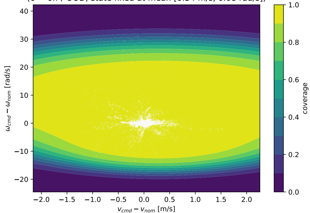
Residual coverage vs command offset (0 = off / OOD; state fixed at mean [0.34 m/s, 0.08 rad/s])
